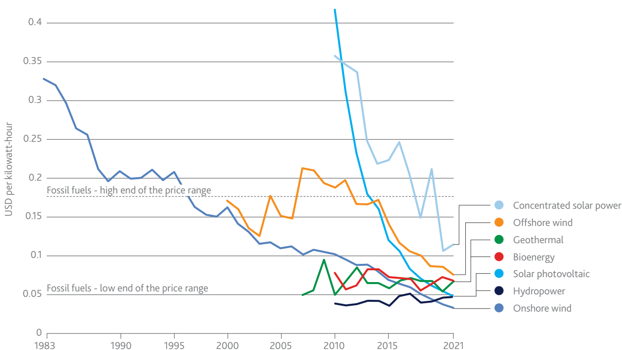
FIGURE 5: LEVELISED COSTS OF RENEWABLE ENERGY SOURCES BY TECHNOLOGY IN RECENT DECADES
